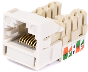
CC0020883/1 | UNJ600-WH Uniprise UNJ600 Category 6 U/UTP Information Outlet, white
