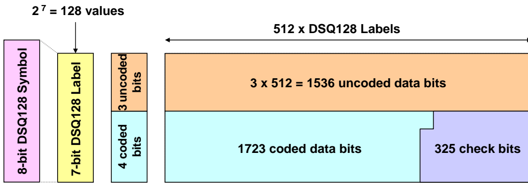
Figure 3: DSQ128 Code block with LDPC (1723, 2048)
